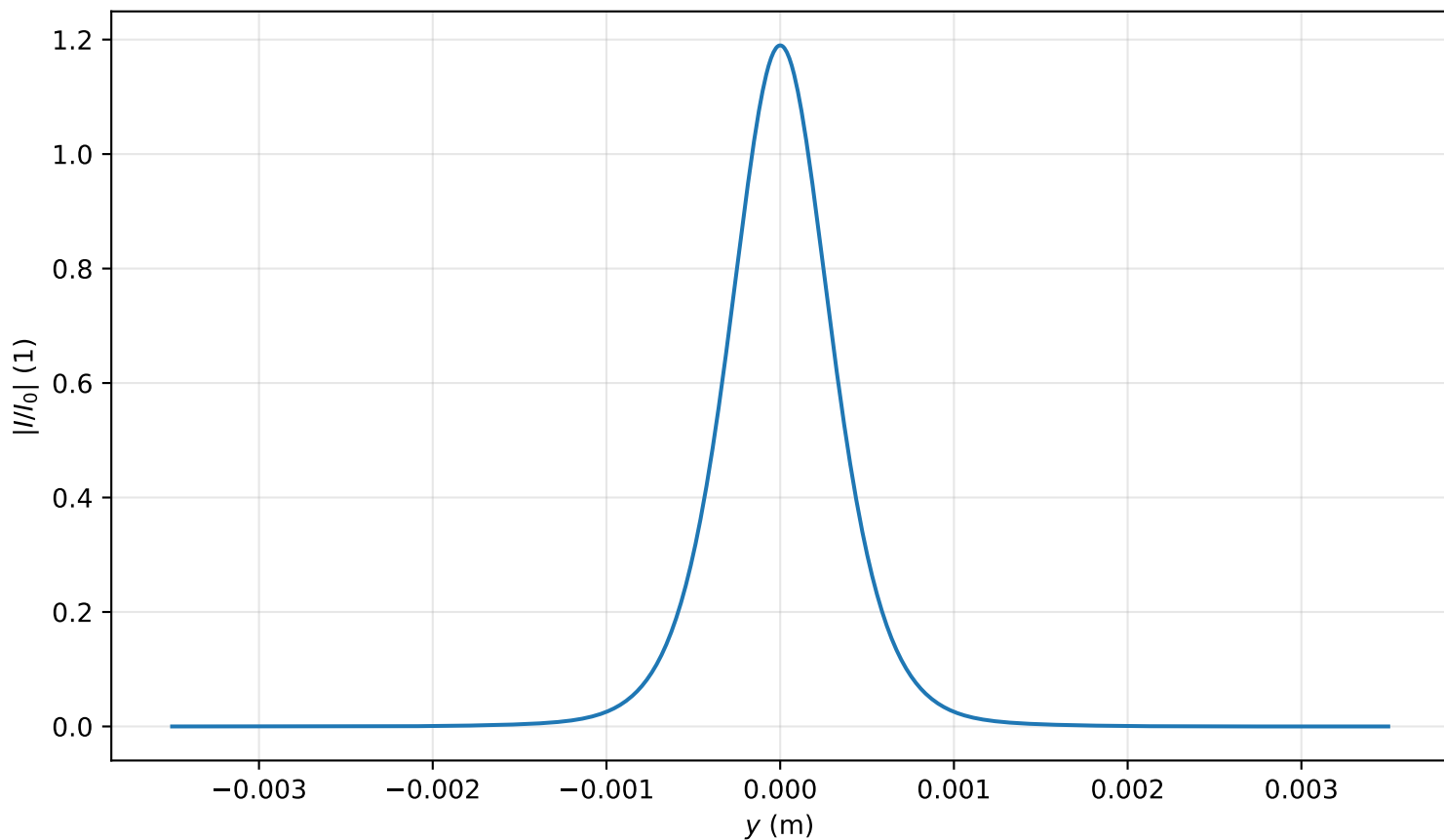
Intensity profile I(x=0, y, z=2.627)/I_0 , P_{in}=0.8P_{cr} , artificial time
